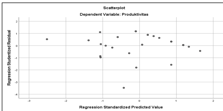
Figure 4. Scatterplot
