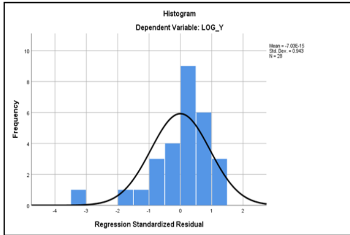
Figure 2. Histogram
